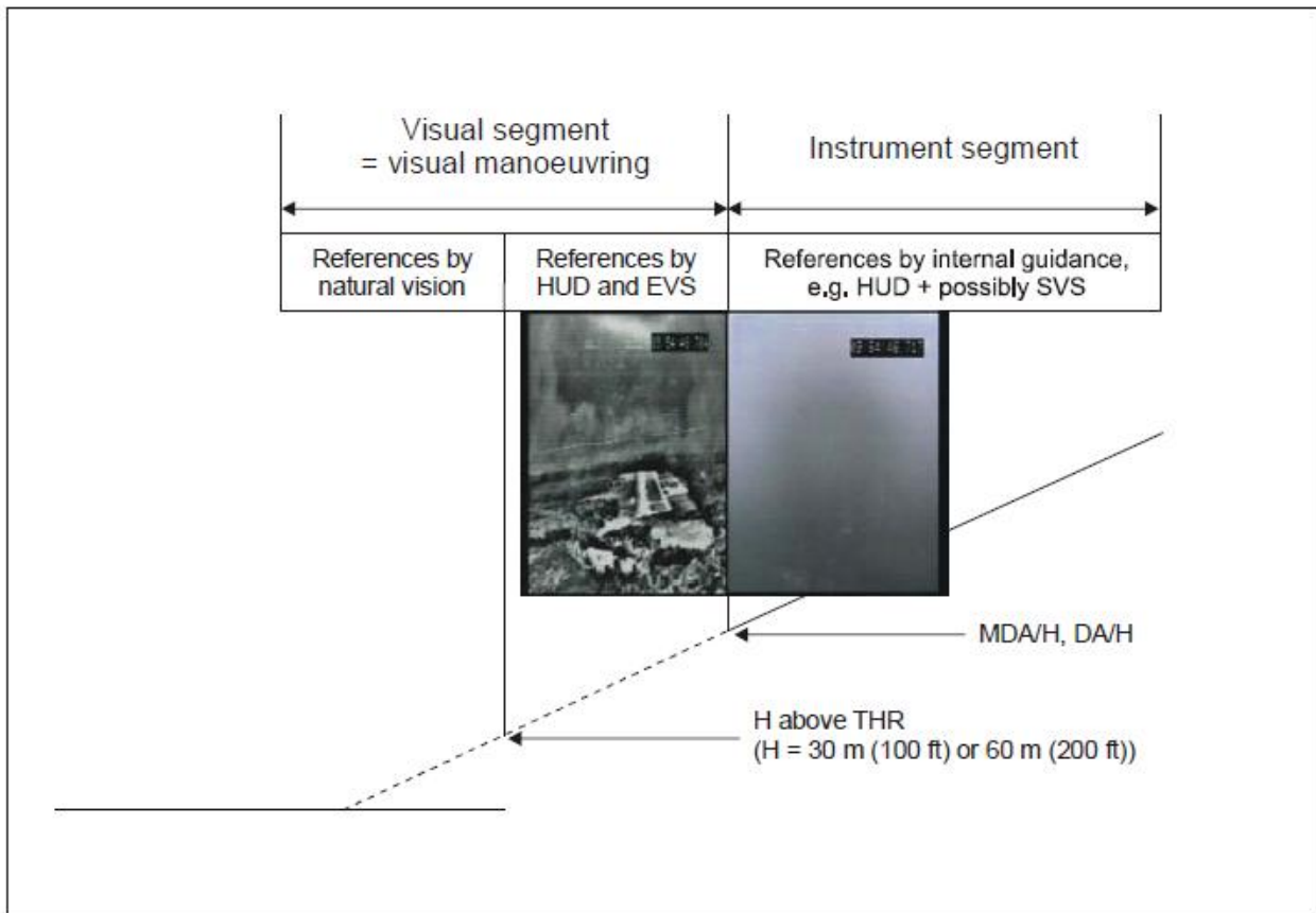
Figure 1-1 EVS Operations- transition from instrument to visual references
